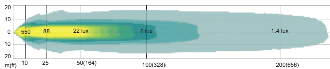
Standard Flood Lens Cover 4082
